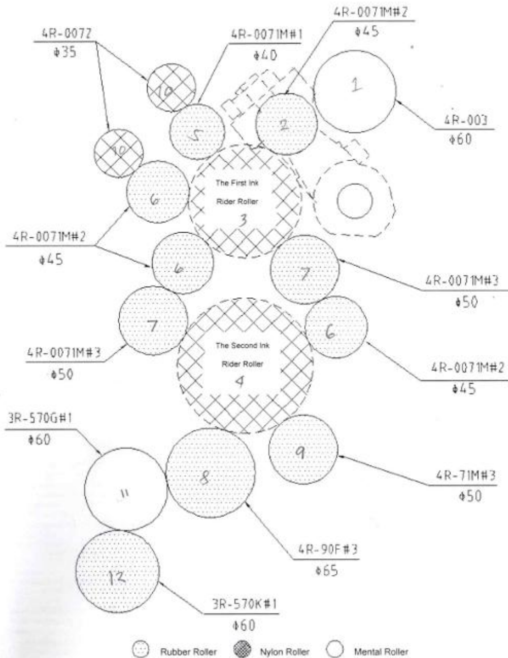
Deployment Diagram of the BA Rubber Roller
